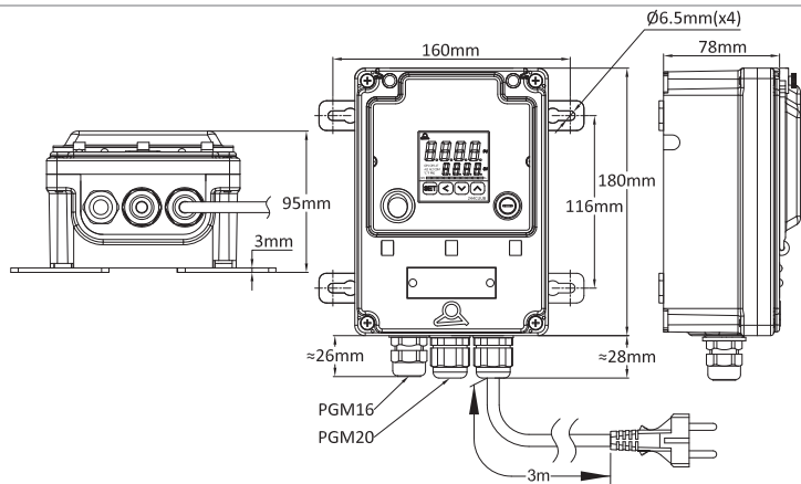
Model with 3 cable glands
