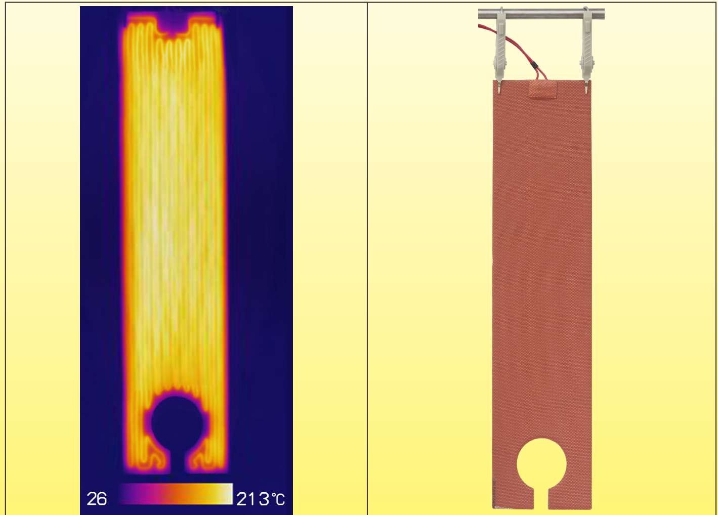
Thermographic image of a 2.4mm flat silicone heater with a 1\text{W}/\text{cm}^2 surface power load, suspended in calm air, not fixed on a board, at an ambient temperature of 25^\circ\text{C} . The surface temperature reaches 213^\circ\text{C} , nearby its destruction.
