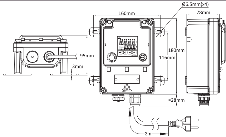
Model with 5 ways waterproof connector
