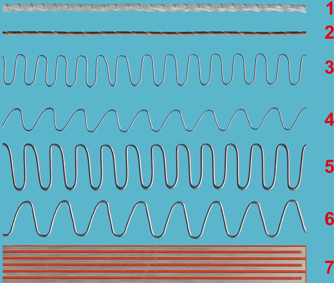
1: Wound around a fiberglass core with 1 to 6 conductors in parallel; 2: Wound around aramid core with 1 to 6 conductors in parallel; 3, 4, 5, 6: Flat zig-zag spring; 7: Heating net made by chemical etching of a metal foil.
