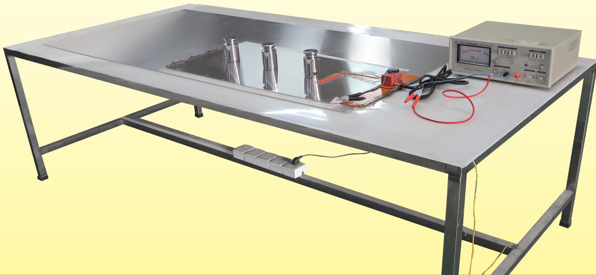
Device for measuring the insulation resistance. The measured values are always greater than 0.1Gohm
